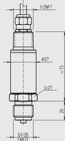
with 1/2 NPT conduit male, with cable outlet
